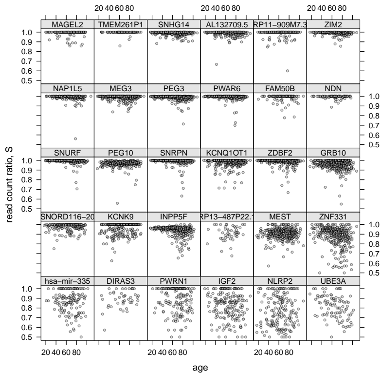
Figure 5: Variation of the read count ratio S_{ig} with age across hundreds of individuals i (dots) and 30 genes g that have been considered as imprinted in the DLPFC brain area in this study.
