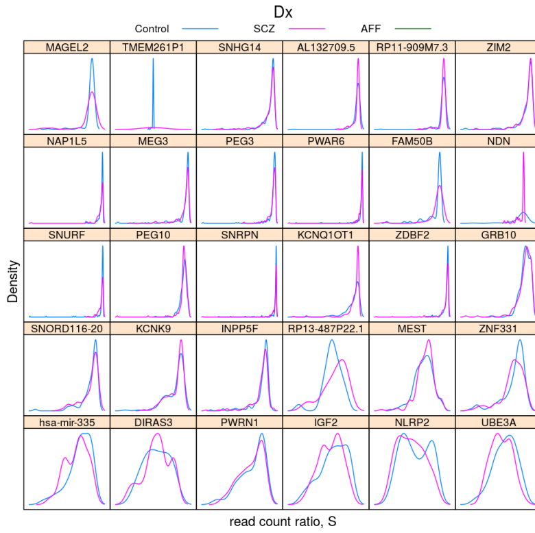
Figure 4: Distribution of read count ratio for control and schizophrenic (SCZ) individuals within each gene.
